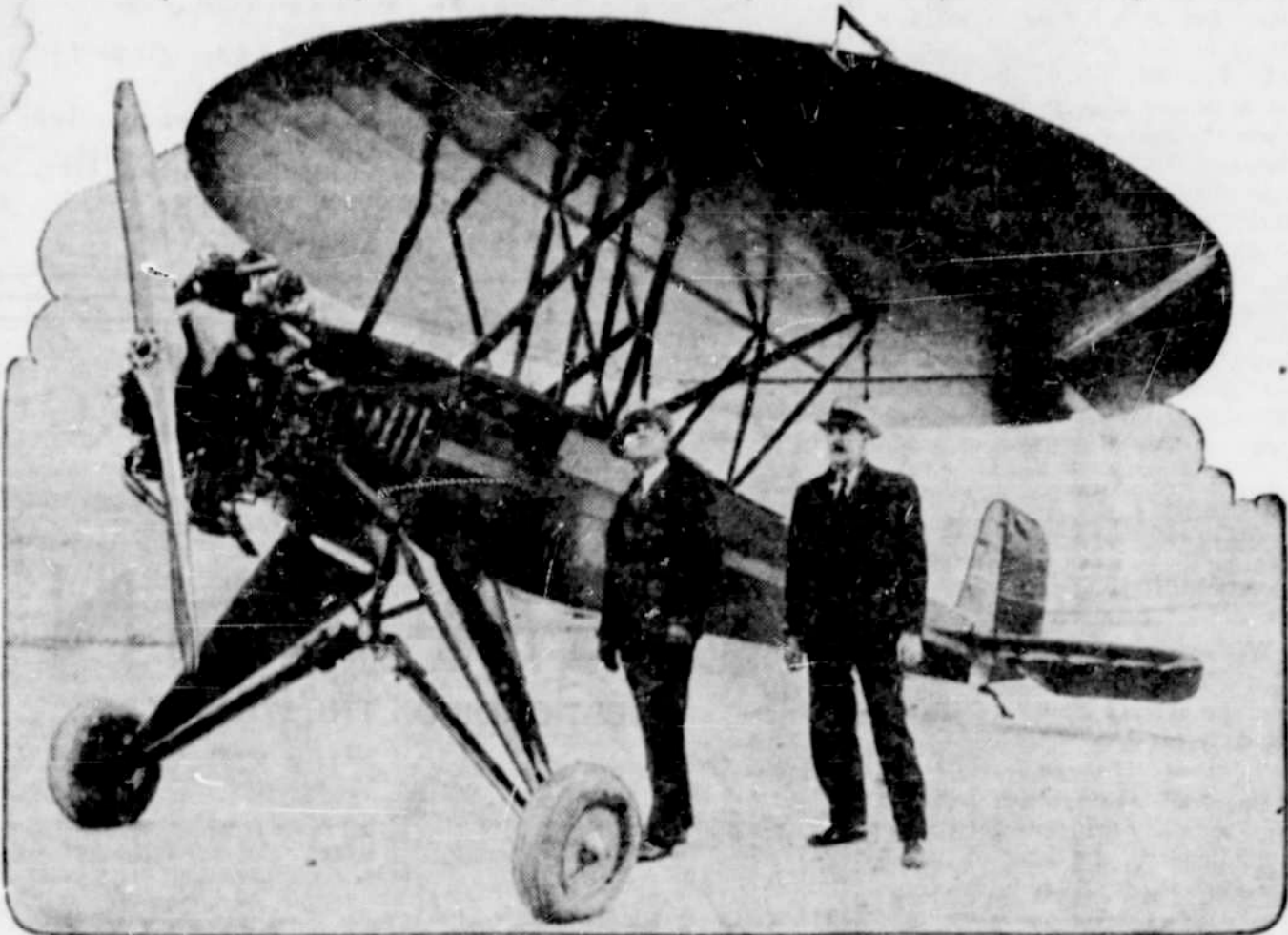
This "Circle Plane" may replace the runabout in the average American family, according to the designers. The plane has an umbrella-like wing and can be landed at a 90-degree angle in a 25-foot area. It can travel 135 miles per hour, and comes down to earth slower than a parachute.
